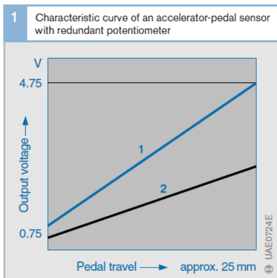
Fig. 1 1 Potentiometer 1 (master potentiometer) 2 Potentiometer 2 (50% of voltage)
